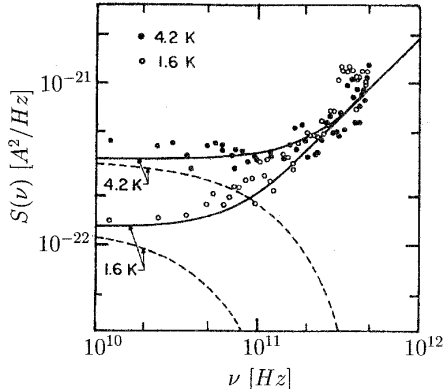
FIG. 1: Spectral density of current noise as measured in [15] for two different temperatures. The solid line is the prediction of eq. (1), while the dashed line neglects the zero-point term.
